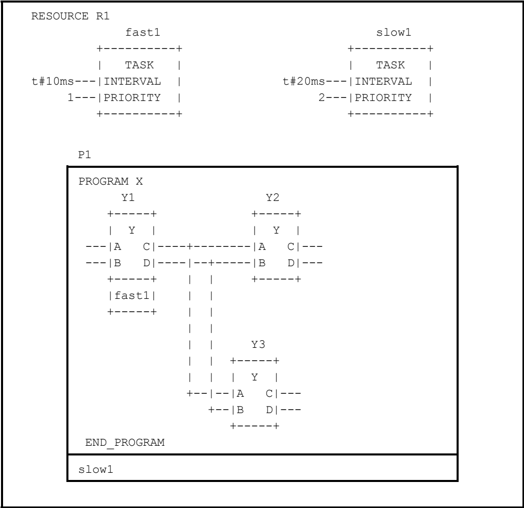
Figure 21 b) - Synchronization of function blocks with implicit task associations
