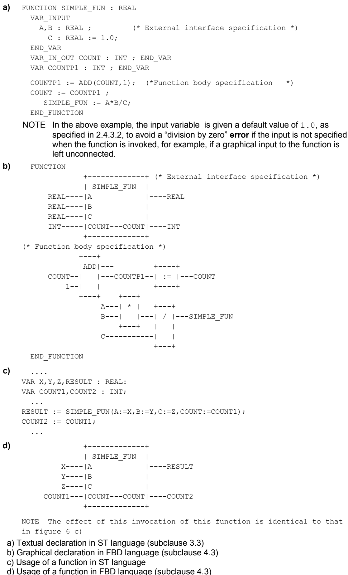
Figure 6 - Examples of function declarations and usage
