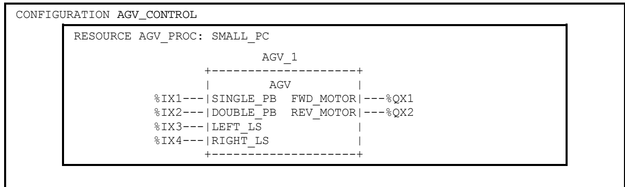
Figure F.11 - A graphical configuration of program AGV
