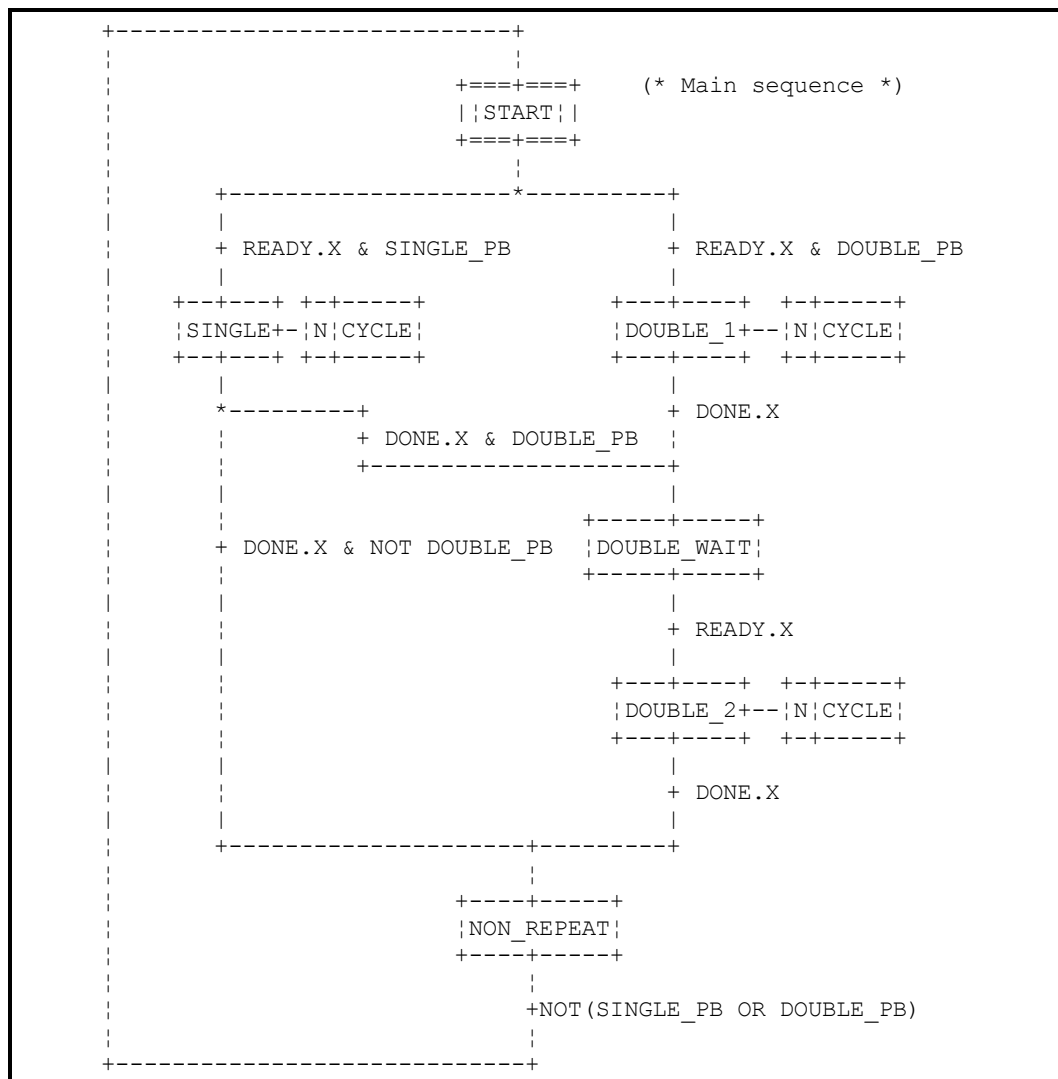
Figure F.12 - Body of program AGV
